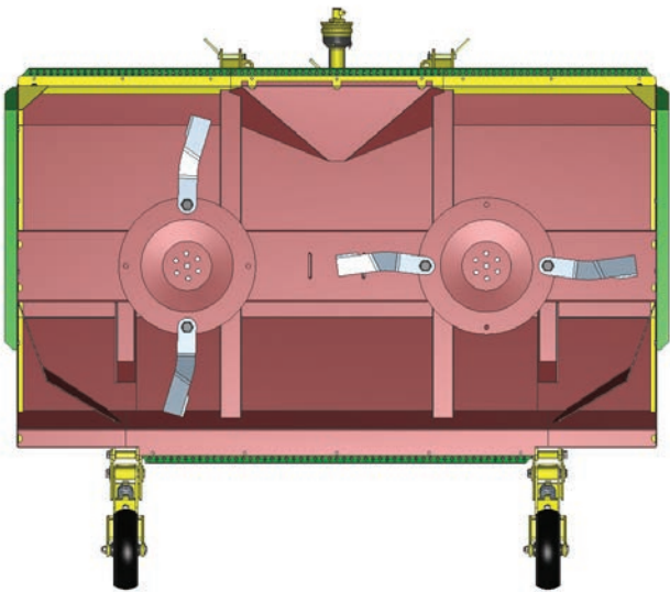
Two round, low-impact blade discs fitted with two 360°-swinging blades on each disc
